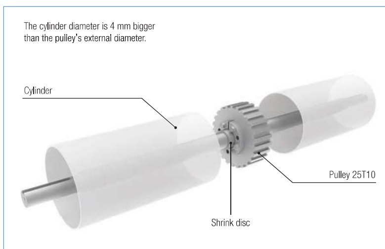
Motor drum principle for timing belt 25T10
