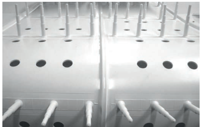
Belts with fingers, profiles and perforations
