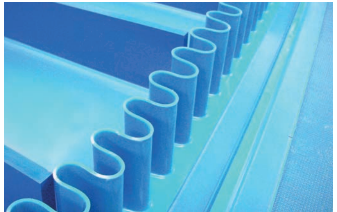
Belts with profiles, cleats and Compart™ Sidewalls
