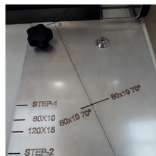
Setting for diagonal finger
