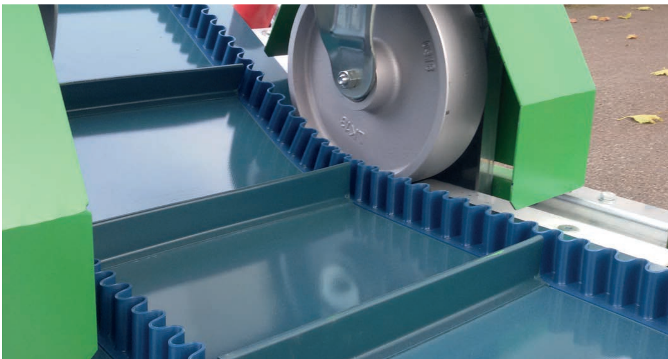
Cross-rigid belt for Z-conveying (swan or goose neck)
